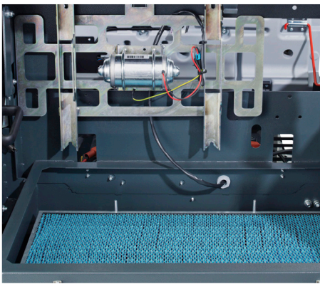
An electrical time Liberatorm™ multi-frequency filter shaker cleans the filter efficiently even in dusty applications
